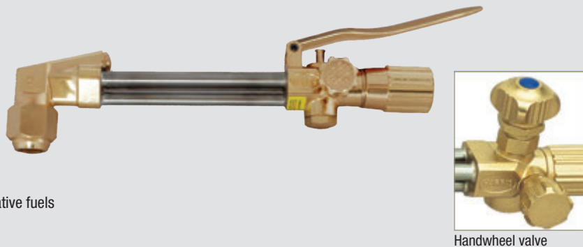
Handwheel valve
